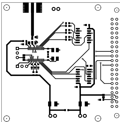
Figure 73 Test Board Layout , Top View
