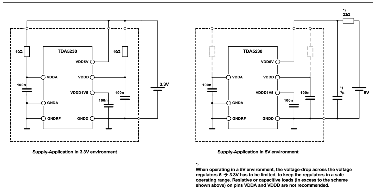
Figure 11 Supply Modes
