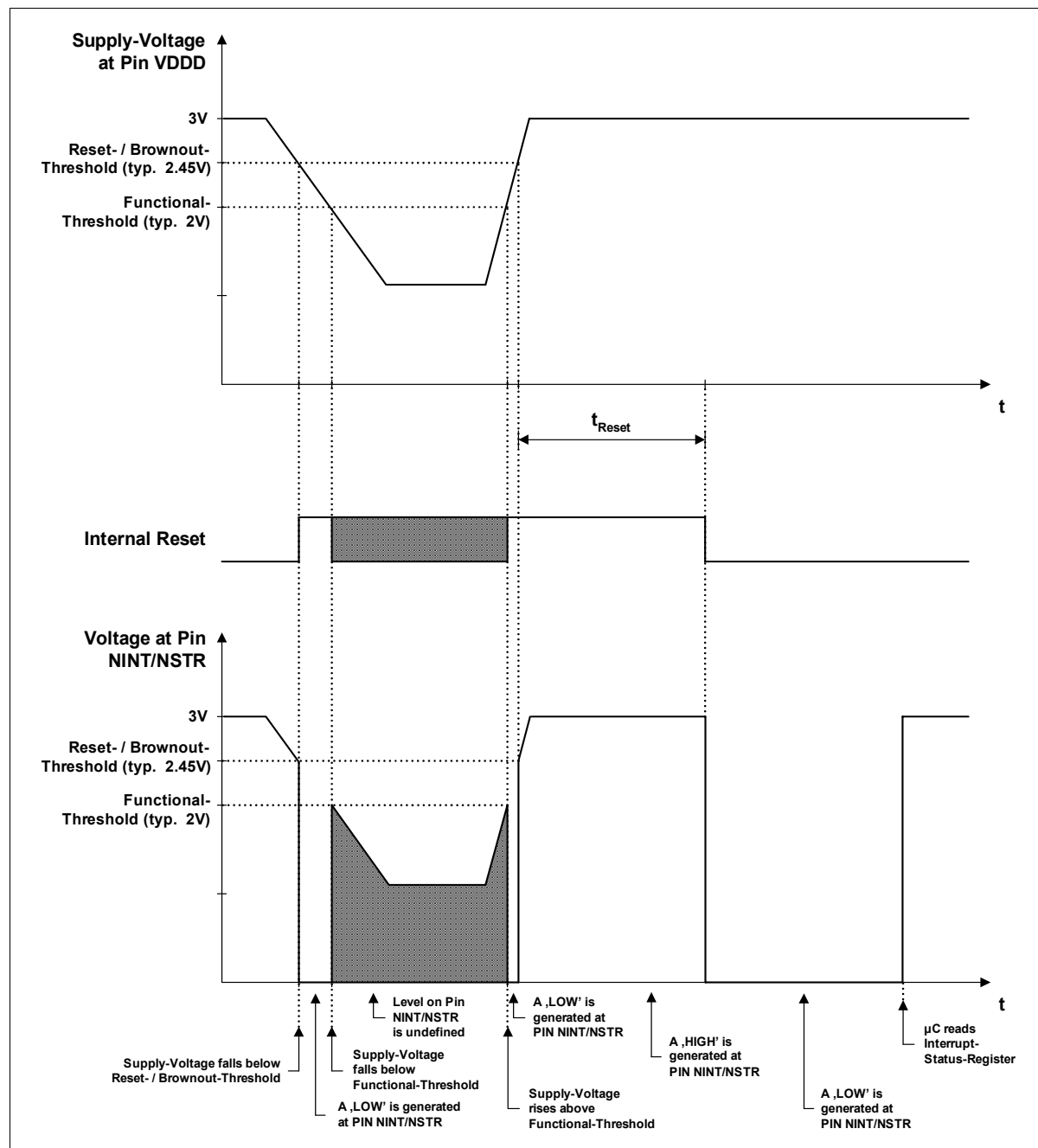
Figure 13 Reset Behavior
