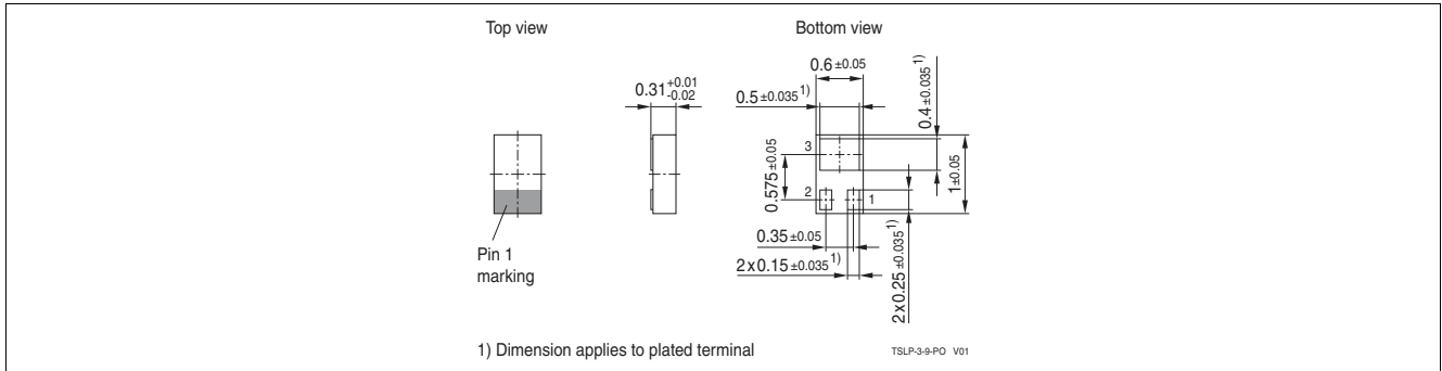
Figure 7-1 Package Outline
