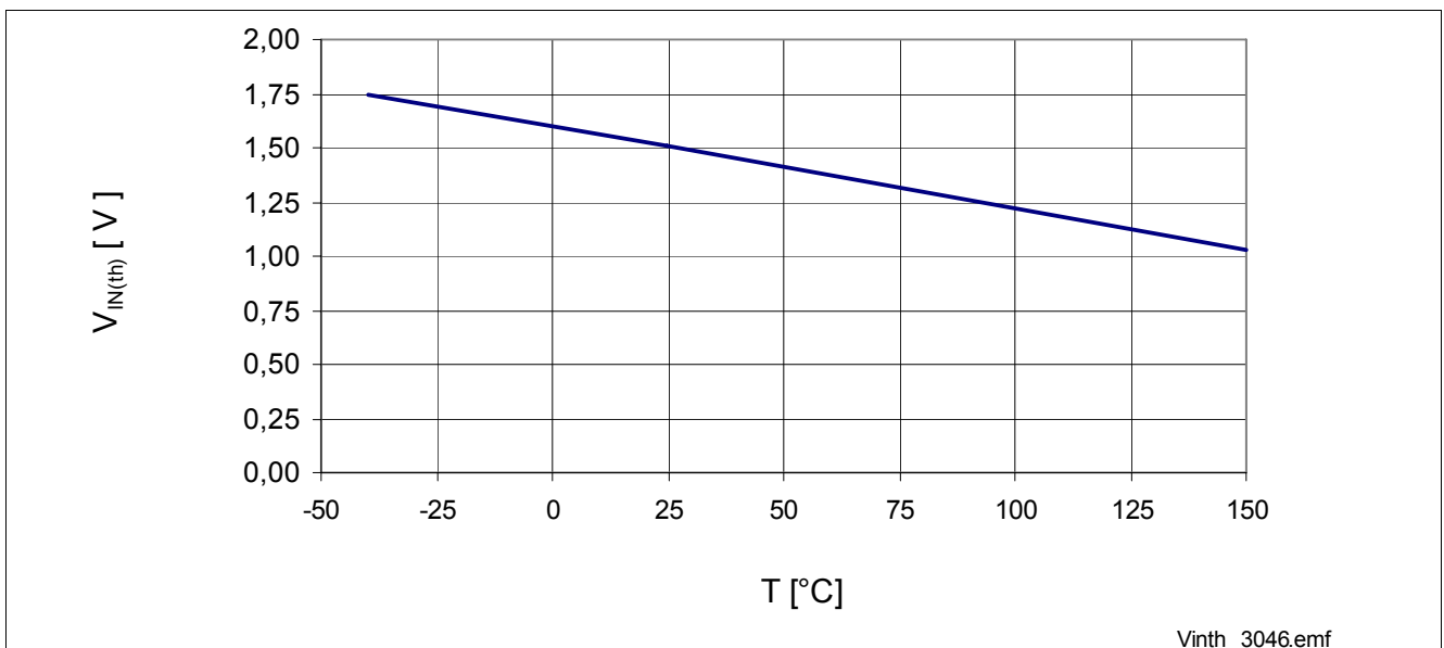
Figure 6 Typical Input Threshold Voltage V_{inth} = f(T_J) ; I_D = 1.2mA , V_D = V_{IN}
