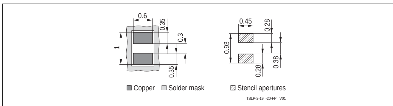
Figure 4-6 TSLP-2-20: Footprint
