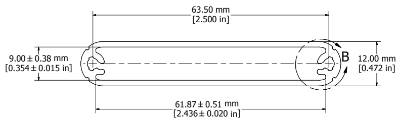
EXTRUSION
