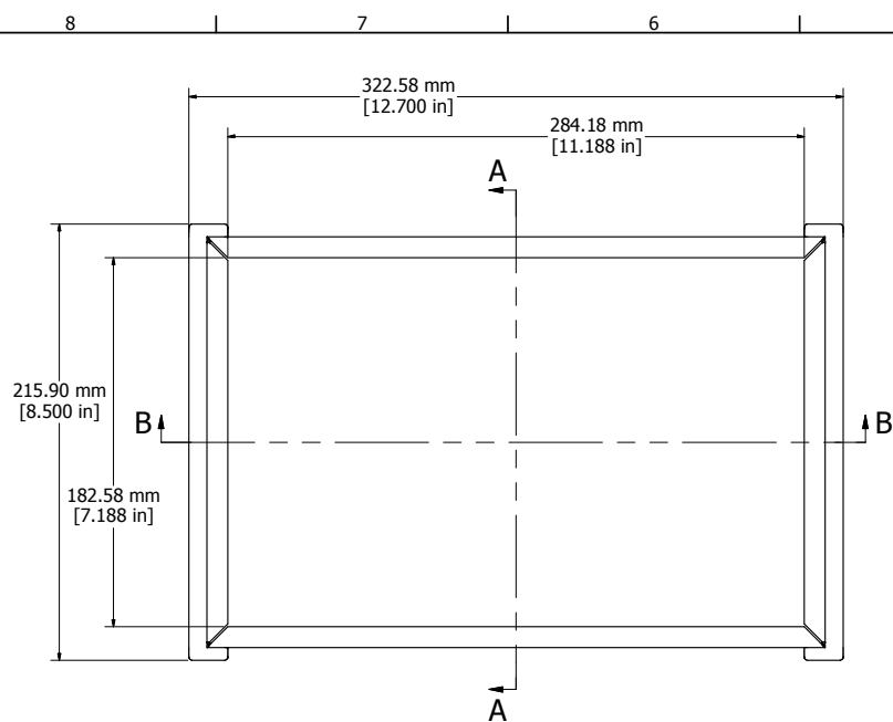
Assembly - View From Bottom
