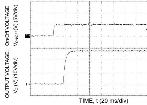
Figure 10. Typical Start-Up Using Remote On/Off, negative logic, C_{o,ext} = 330\mu F .
