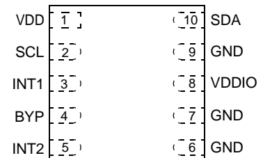
Pin Connections
