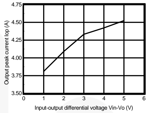
Figure 37. Output Peak Current vs. Input-Output Differential Voltage
