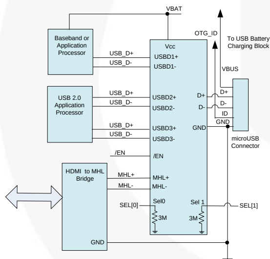
Figure 1. Typical Application
