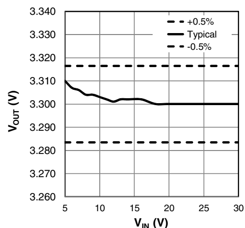
Figure 2: Line regulation
