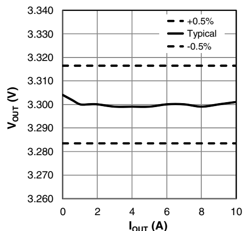
Figure 1: Load Regulation
