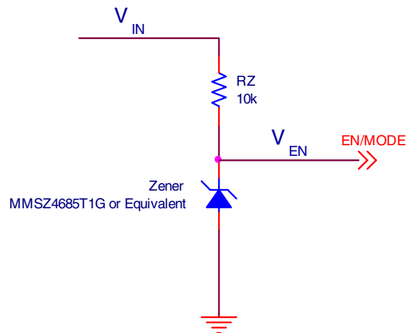
Figure 19: Selecting DCM/CCM by deriving EN/MODE from VIN
