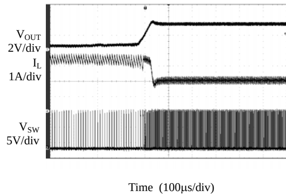
Figure 13. Short Circuit Recovery ( I_{OUT}=2\text{A} )
