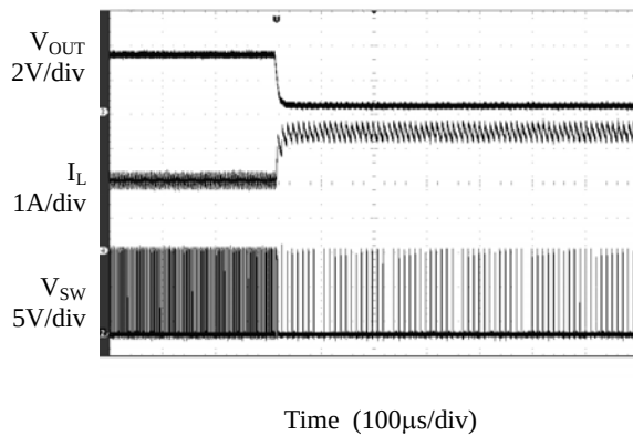
Figure 12. Short Circuit Protection ( I_{OUT}=2\text{A} )
