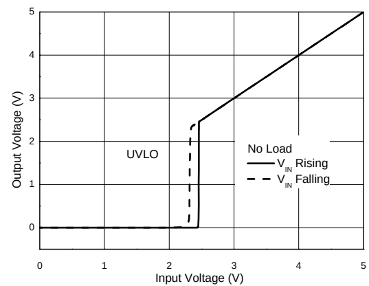
Figure 9. UVLO Function
