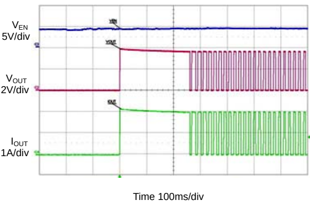
Figure 29. Thermal Shutdown Response ( V_{IN}=5.0V , C_{OUT}=4.7\mu F , R_L=1.65\Omega )
