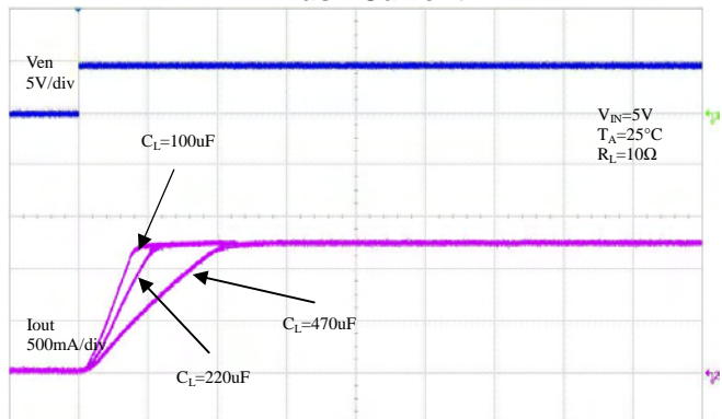
Inrush Current
