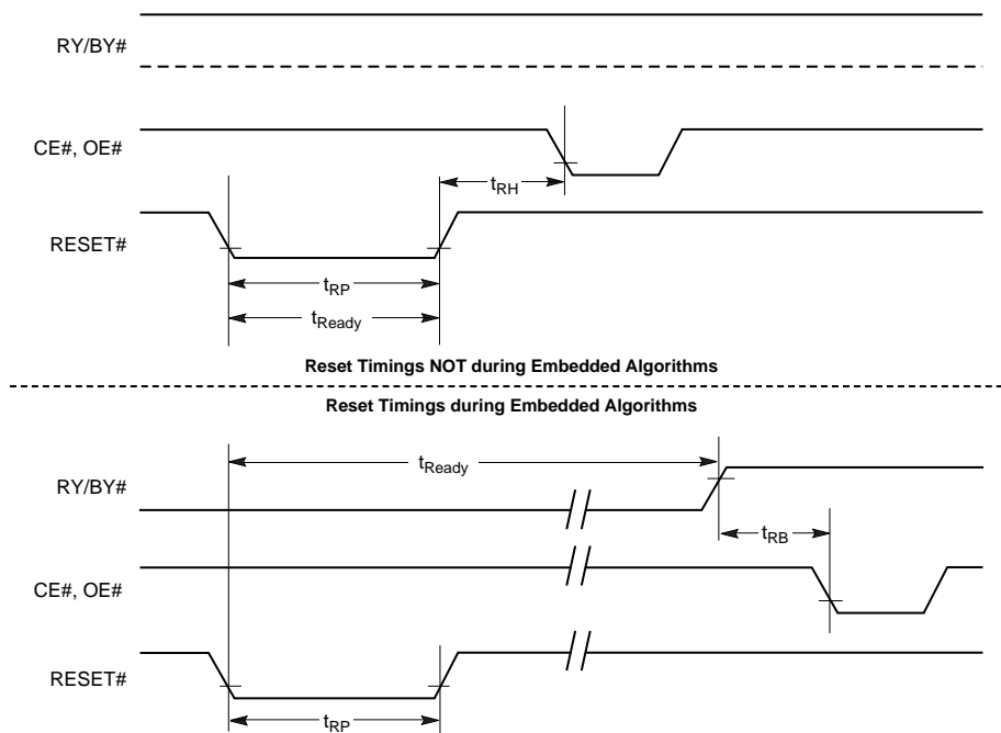
Figure 17.2 Reset Timings
