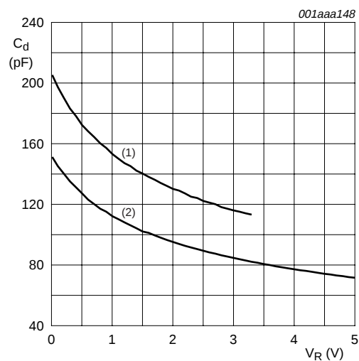
f = 1\text{ MHz} ; T_{amb} = 25\text{ }^{\circ}C (1) PESD3V3S1UB (2) PESD5V0S1UB
