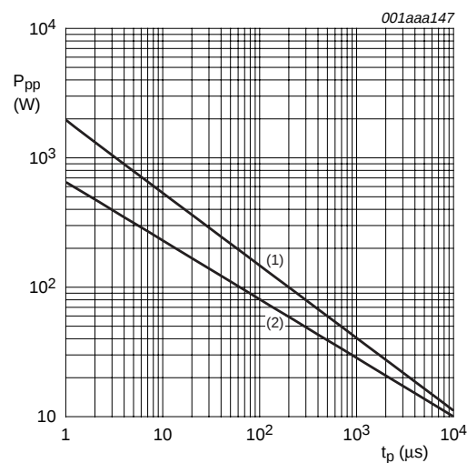
T_{amb} = 25\text{ }^{\circ}C t_p = 8/20\text{ }\mu s exponentially decay waveform, see Figure 1 (1) PESD3V3S1UB and PESD5V0S1UB (2) PESD12VS1UB, PESD15VS1UB; PESD24VS1UB
