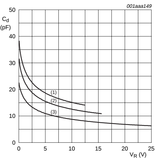
f = 1\text{ MHz} ; T_{amb} = 25\text{ }^{\circ}C (1) PESD12VS1UB (2) PESD15VS1UB (3) PESD24VS1UB
