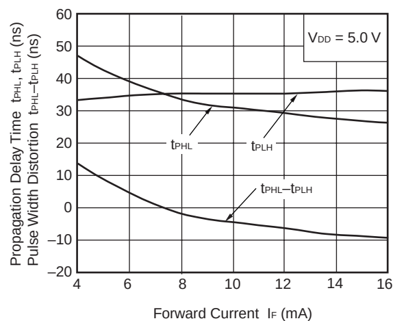
t_{PHL} , t_{PLH} , t_{PHL}-t_{PLH} vs. FORWARD CURRENT
