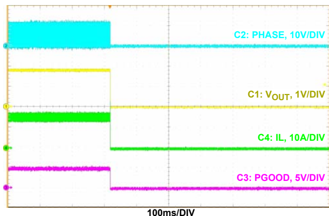
FIGURE 26. LATCH-OFF OCP ( V_{IN} = 12V , V_{OUT} = 1.8V , 600kHz)
