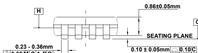
SIDE VIEW 1
