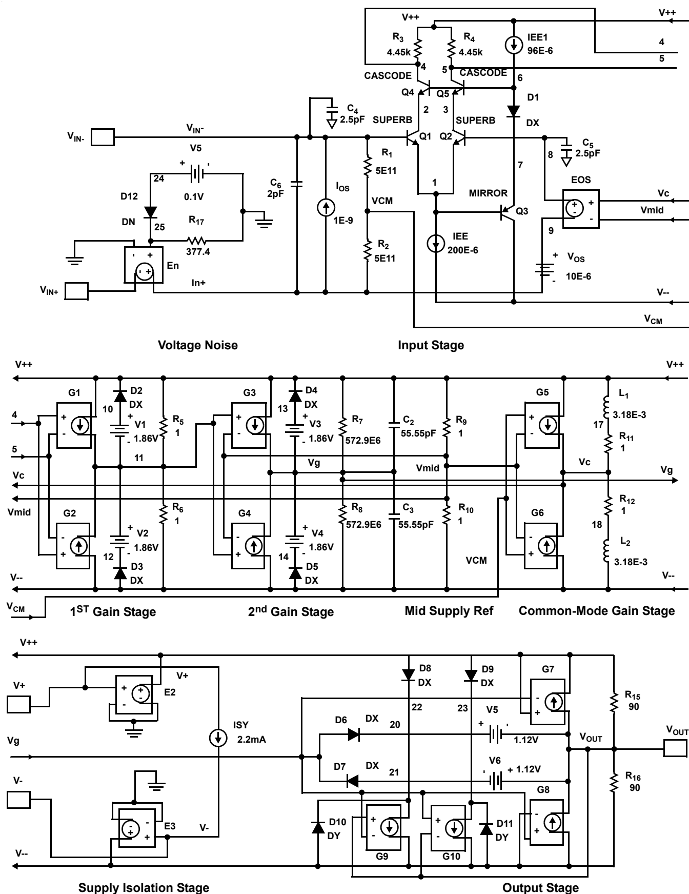
FIGURE 41. SPICE SCHEMATIC
