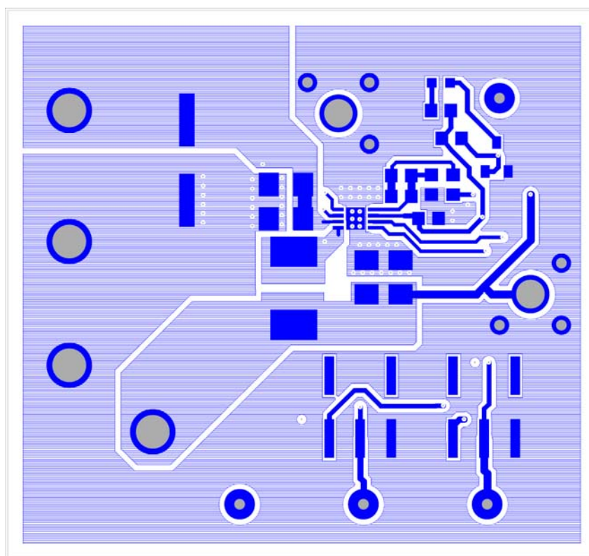
FIGURE 4. TOP LAYER COMPONENT SIDE
