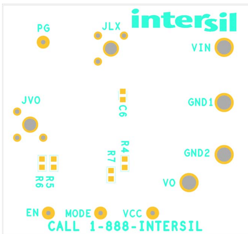
FIGURE 8. SILK SCREEN BOTTOM
