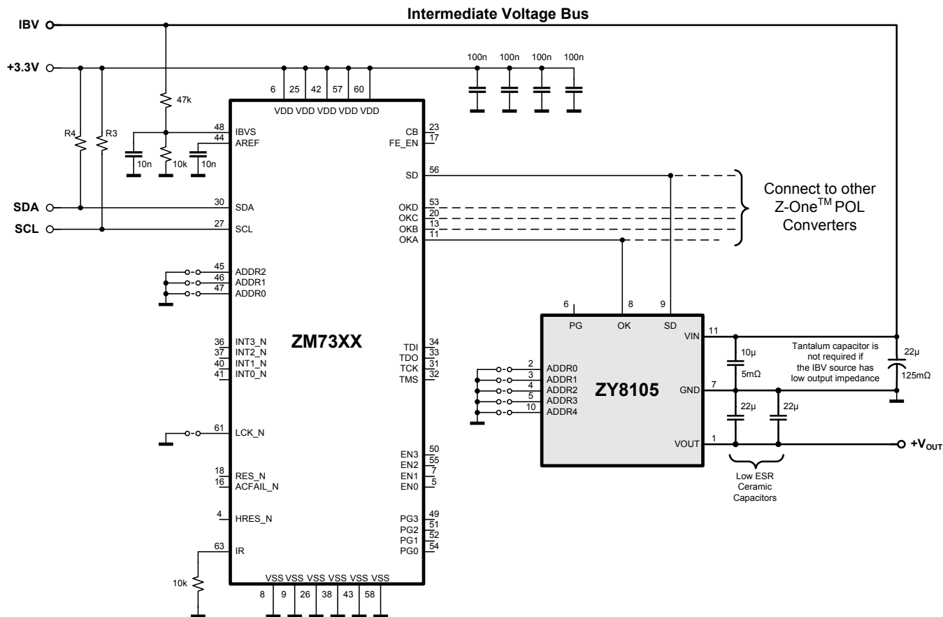
Figure 16. Block Diagram of Typical Application with Digital Power Manager and I 2 C Interface
