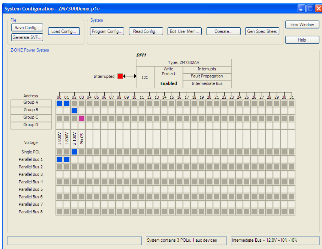
Figure 43. GUI System Configuration Window
