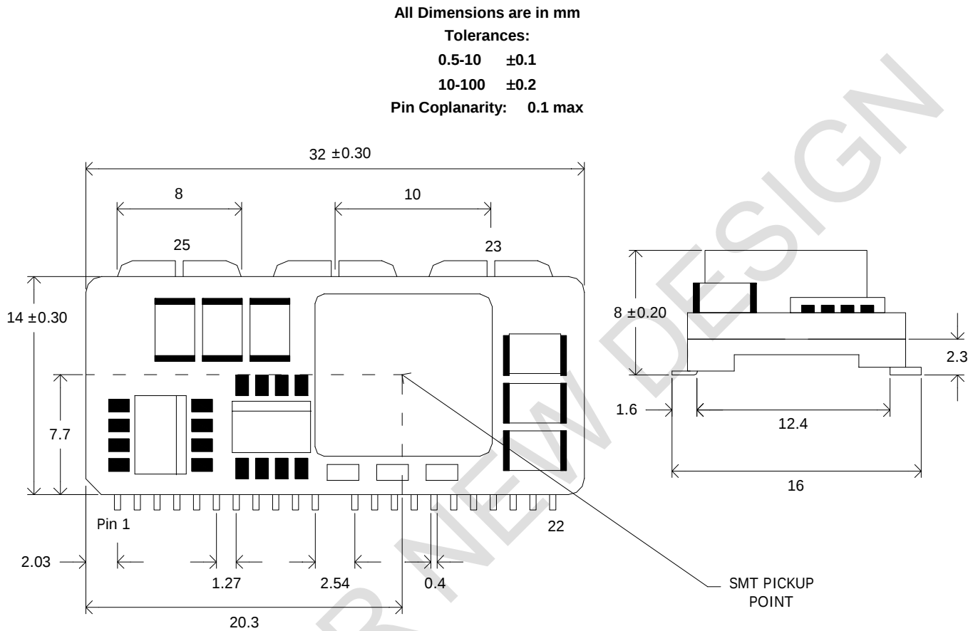
Figure 20. Mechanical Drawing
