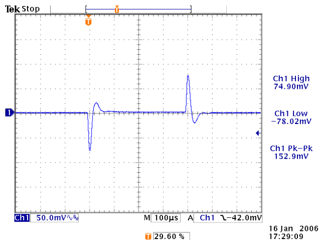
Figure 9. Vin=12V, Vout=1V. CCA=07
