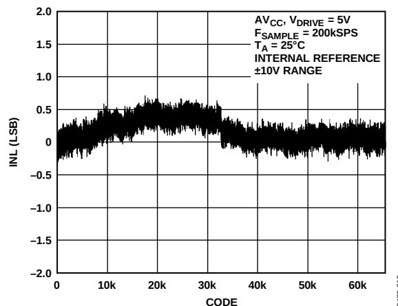
Figure 14. AD7606 Typical INL, \pm 10 V Range
