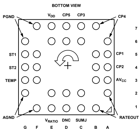
Figure 3. Pin Configuration
