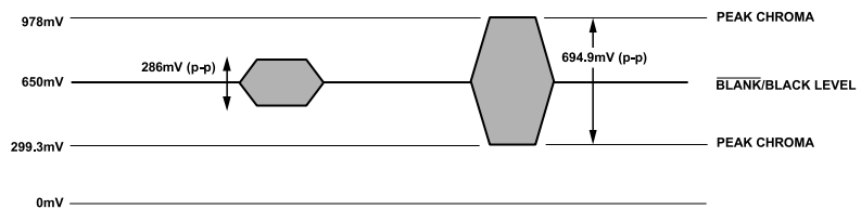
Figure 67. NTSC Chroma Video Levels
