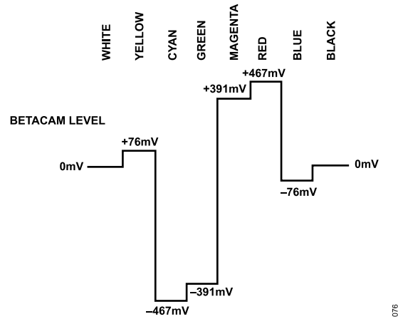
Figure 77. NTSC 100% Color Bars with Pedestal Pr Levels
