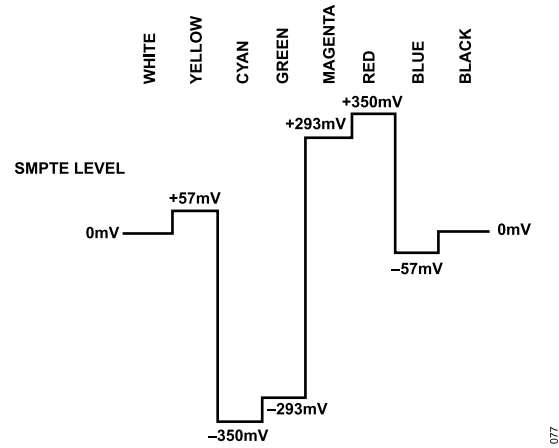
Figure 78. PAL 100% Color Bars, Pr Levels
