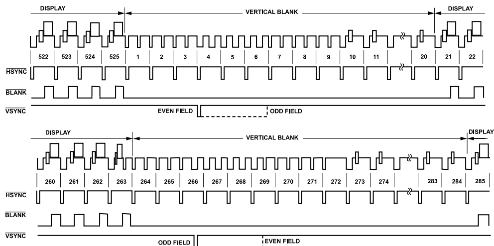
Figure 27. Timing Mode 2 (NTSC)
