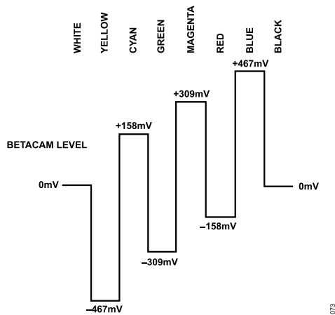
Figure 74. NTSC 100% Color Bars with Pedestal Pb Levels
