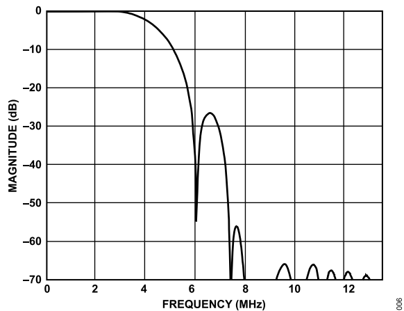
Figure 6. Chrominance Internal Filter Specifications
