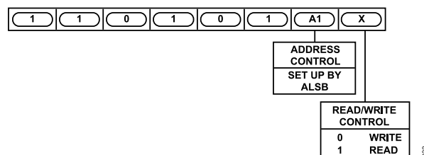
Figure 33. ADV7174 Subordinate Address
