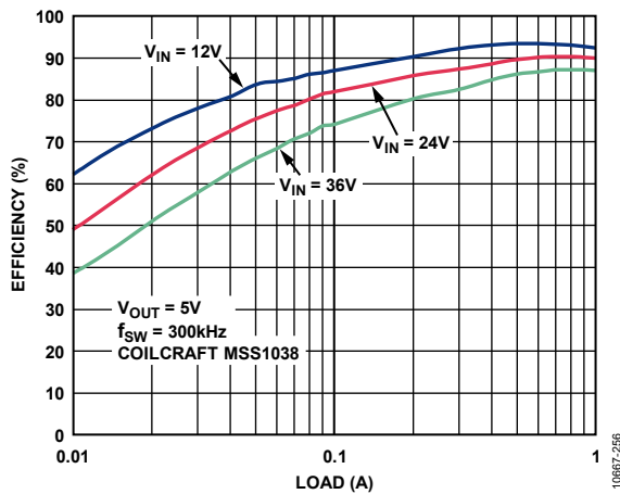
Figure 11. Efficiency vs. Load Current, V_{OUT} = 5\text{ V} , f_{SW} = 300\text{ kHz}
