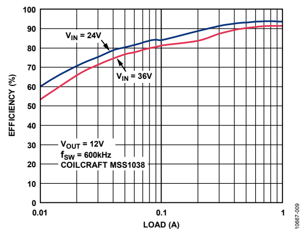
Figure 15. Efficiency vs. Load Current, V_{OUT} = 12\text{ V} , f_{SW} = 600\text{ kHz}
