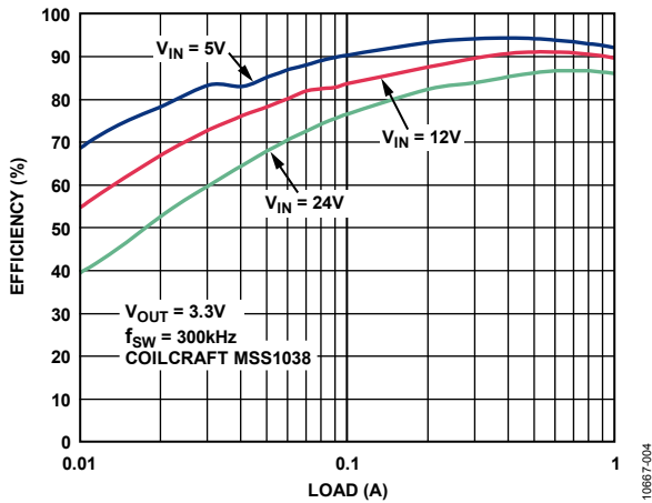
Figure 10. Efficiency vs. Load Current, V_{OUT} = 3.3\text{ V} , f_{SW} = 300\text{ kHz}
