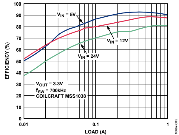
Figure 13. Efficiency vs. Load Current, V_{OUT} = 3.3\text{ V} , f_{SW} = 700\text{ kHz}
