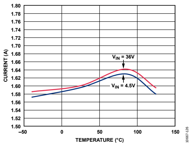
Figure 31. Current Limit vs. Temperature
