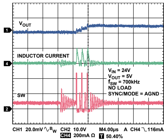
Figure 33. Pulse Skip Mode, V_{IN} = 24V , V_{OUT} = 5V , f_{SW} = 700kHz , No Load, SYNC/MODE = AGND
