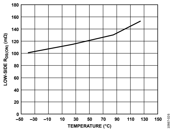
Figure 32. Low-Side R_{DS(ON)} vs. Temperature
