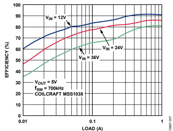
Figure 14. Efficiency vs. Load Current, V_{OUT} = 5\text{ V} , f_{SW} = 700\text{ kHz}
