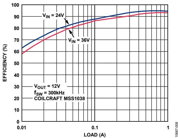
Figure 12. Efficiency vs. Load Current, V_{OUT} = 12\text{ V} , f_{SW} = 300\text{ kHz}
