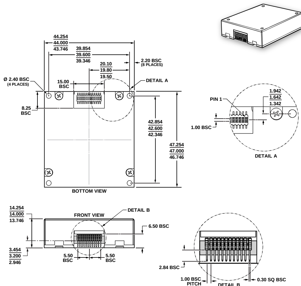
Figure 31. 24-Lead Module with Connector Interface [MODULE] (ML-24-6)
