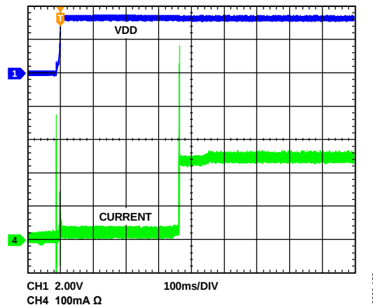
Figure 29. Transient Current Demand, Start-Up
