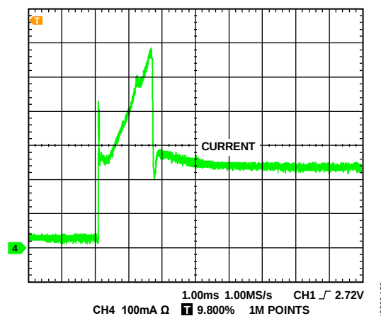
Figure 30. Transient Current Demand, Peak Demand
