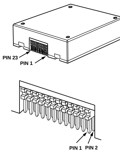
Figure 6. Axial Orientation (Top Side Facing Up)
