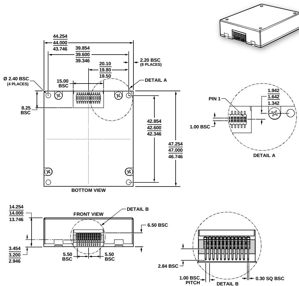
Figure 32. 24-Lead Module with Connector Interface [MODULE] (ML-24-6)
