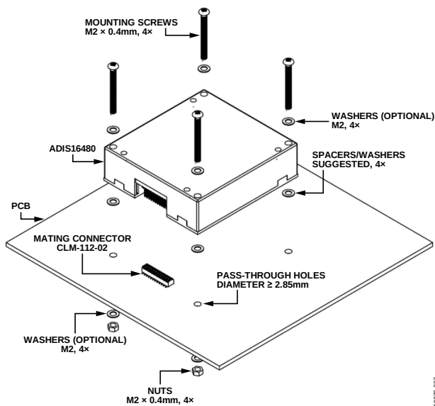
Figure 27. Mounting Example
