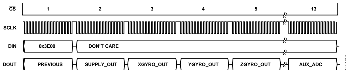
Figure 11. Burst Mode Read Sequence
