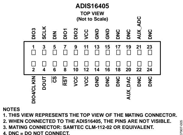
Figure 5. Pin Configuration
