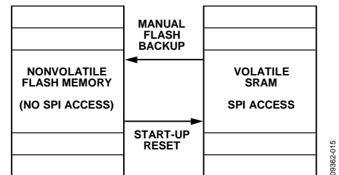
Figure 17. SRAM and Flash Memory Diagram
