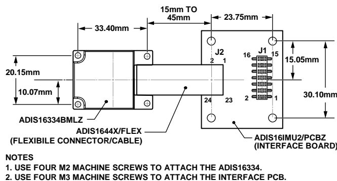
Figure 24. Physical Diagram for ADIS16334 Accessories
