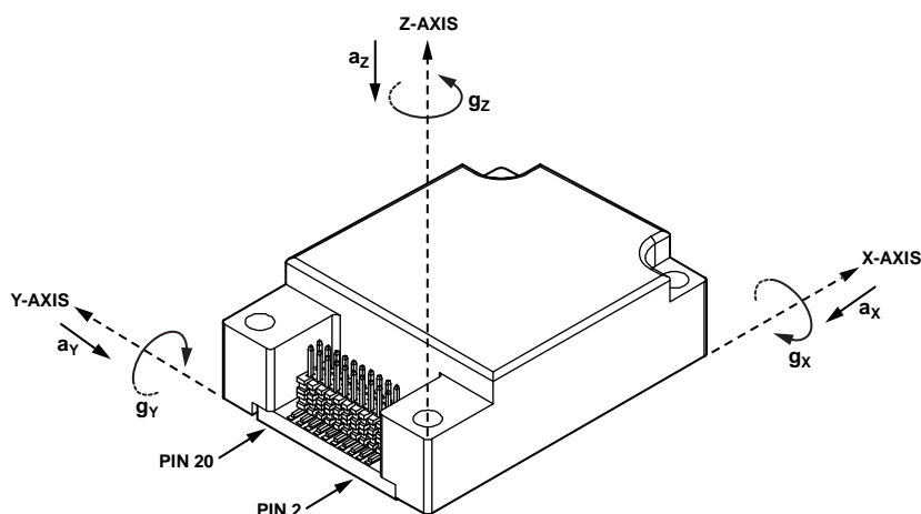
Figure 5. Pin Configuration
