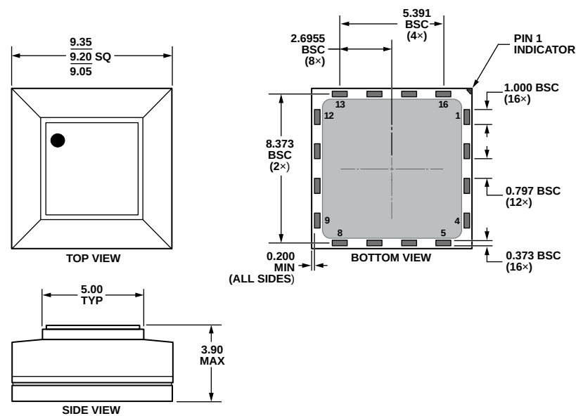
Figure 34. 16-Terminal Land Grid Array [LGA] (CC-16-2) Dimensions shown in millimeters
