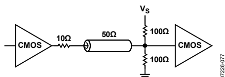
Figure 27. CMOS Output with Far-End Termination
