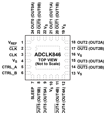
Figure 2. Pin Configuration
