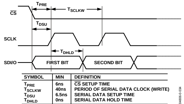
Figure 33. Timing Diagram for Data Write to AD9956
