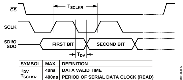
Figure 34. Timing Diagram for Data Read to AD9956
