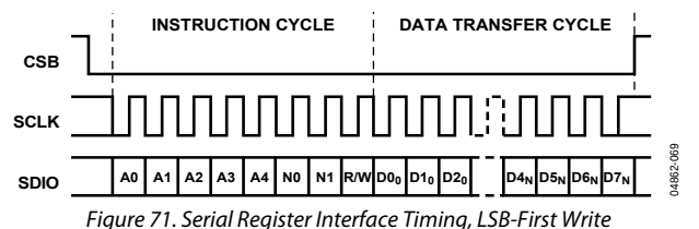
Figure 71. Serial Register Interface Timing, LSB-First Write
