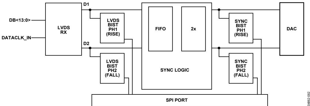
Figure 84. Block Diagram Showing LVDS and SYNC Phase 1 and SYNC Phase 2
