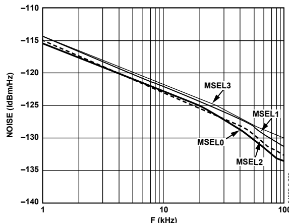
Figure 87. 1/f Noise with Respect to MSEL Bits
