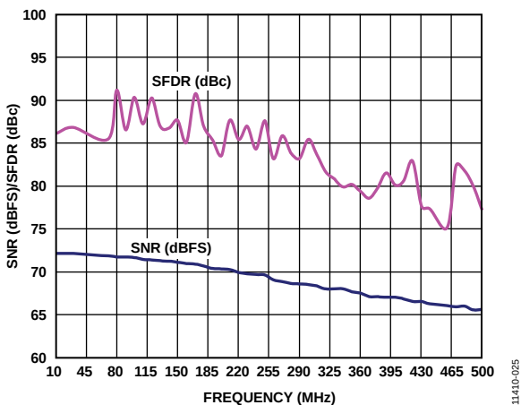
Figure 25. AD9683-250 Single-Tone SNR/SFDR vs. Input Frequency ( f_{IN} )
