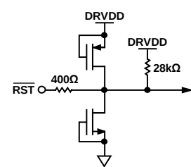
Figure 41. Equivalent \overline{RST} Input Circuit
