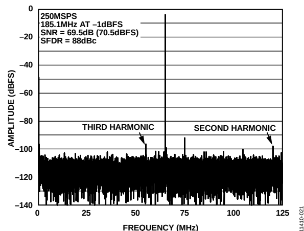
Figure 21. AD9683-250 Single-Tone FFT with f_{IN} = 185.1 MHz
