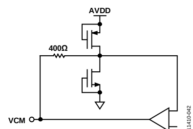
Figure 42. Equivalent VCM Circuit
