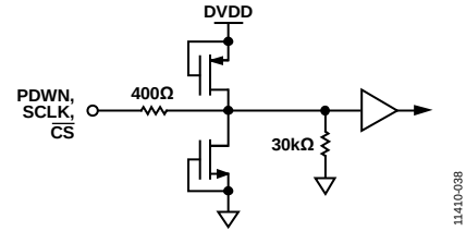
Figure 38. Equivalent PDWN, SCLK, or \overline{CS} Input Circuit
