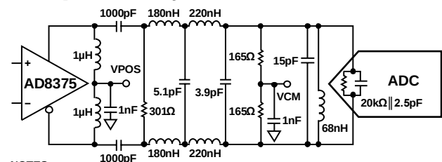
Figure 47. Differential Input Configuration Using the AD8375
