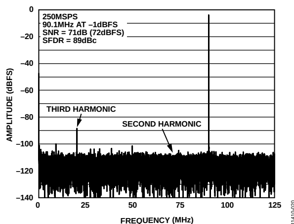
Figure 20. AD9683-250 Single-Tone FFT with f_{IN} = 90.1 MHz, RFCLK = 1.0 GHz with Divide by 4 (Address 0x09 = 0x21)
