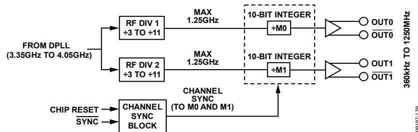
Figure 43. Clock Distribution Block Diagram
