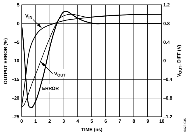
Figure 25. Settling Time
