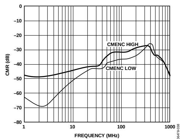
Figure 31. Common-Mode Rejection
