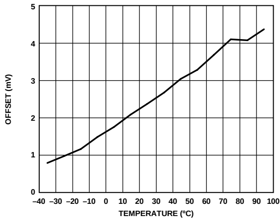
Figure 49. AD8117 V_{OS} vs. Temperature in Broadcast Mode
