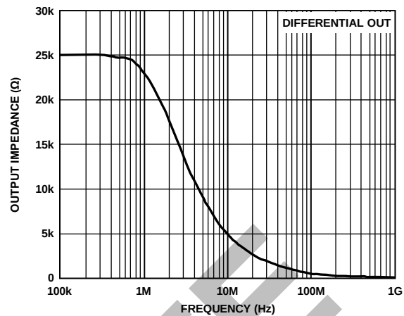
Figure 40. AD8117, AD8118 Output Impedance, Disabled
