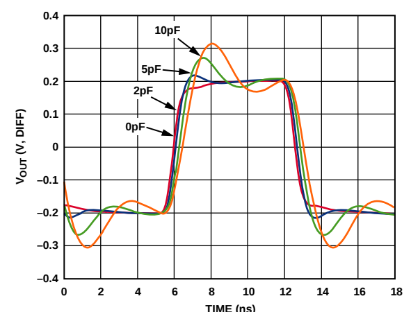
Figure 54. AD8117 Small Signal Pulse Response with Capacitive Loads
