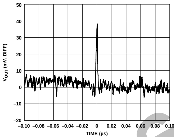
Figure 50. AD8117 Switching Transient (Glitch)
