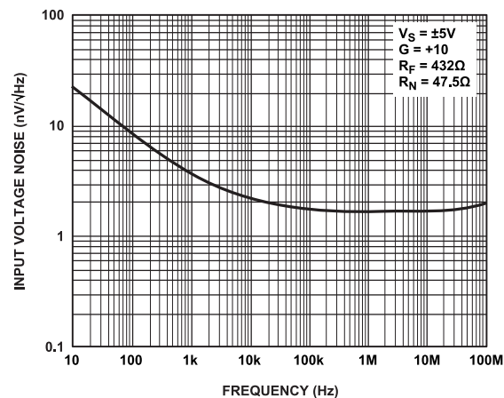
Figure 40. Input Voltage Noise
