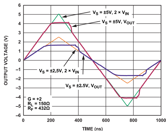
Figure 39. Output Overdrive
