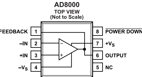
Figure 2. 8-Lead AD8000, 3 mm × 3 mm LFCSP (CP-8-13)
