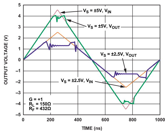
Figure 38. Input Overdrive
