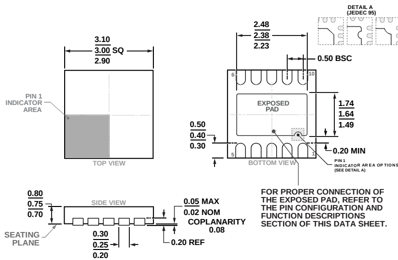
Figure 45. 10-Lead Lead Frame Chip Scale Package [LFCSP] 3 mm × 3 mm Body and 0.75 mm Package Height (CP-10-9)
