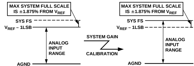
Figure 27. System Gain Calibration
