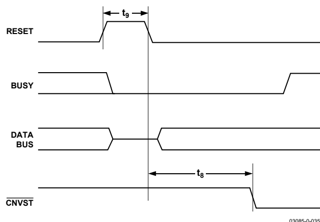
Figure 34. RESET Timing
