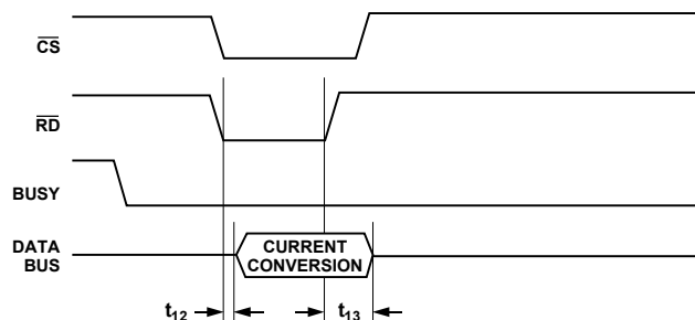
Figure 36. Slave Parallel Data Timing for Reading (Read after Convert)
