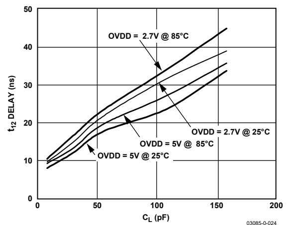
Figure 23. Typical Delay vs. Load Capacitance C_L
