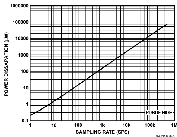
Figure 32. Power Dissipation vs. Sample Rate
