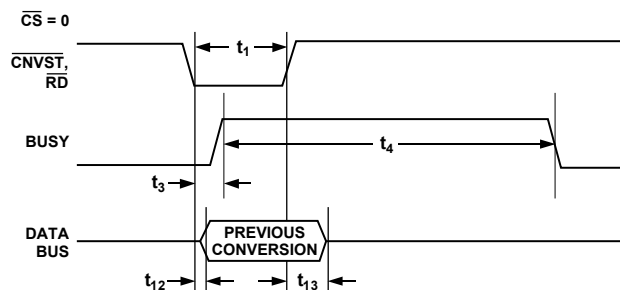
Figure 37. Slave Parallel Data Timing for Reading (Read during Convert)
