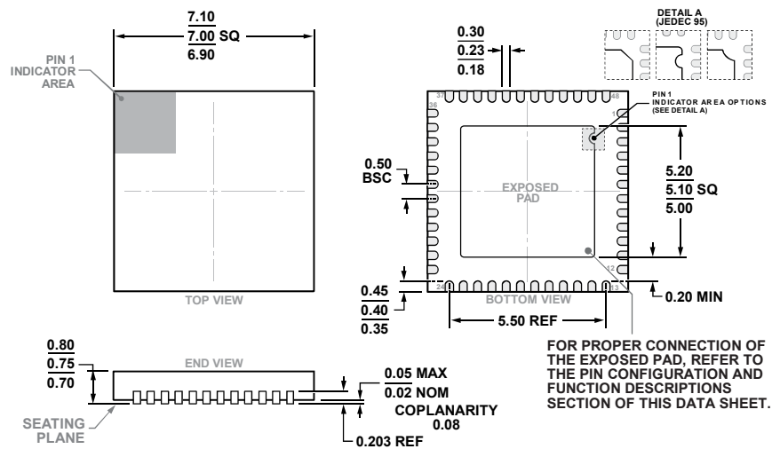
Figure 46. 48-Lead Lead Frame Chip Scale Package [LFCSP] 7 mm × 7 mm Body and 0.75 mm Package Height (CP-48-4) Dimensions shown in millimeters
