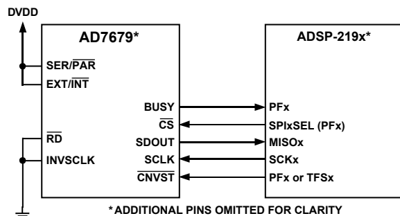
Figure 44. Interfacing the AD7679 to an SPI Interface
