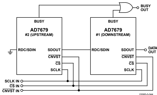
Figure 43. Two AD7679s in a Daisy-Chain Configuration
