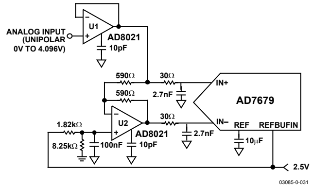
Figure 30. Single-Ended-to-Differential Driver Circuit (Internal Reference Buffer Used)
