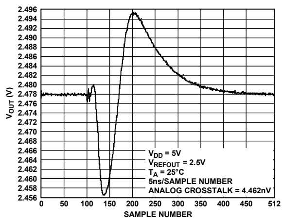
Figure 44. Analog Crosstalk, Internal Reference
