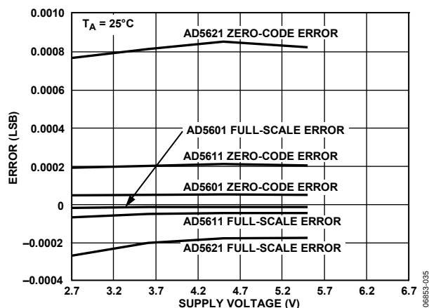
Figure 36. Zero-Code Error and Full-Scale Error vs. Supply Voltage at 25°C
