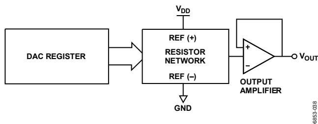
Figure 39. DAC Architecture
