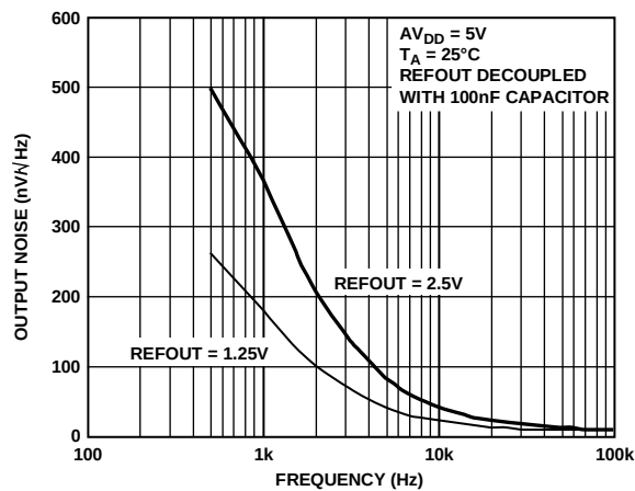
Figure 28. AD5390/AD5391/AD5392 REFOUT Noise Spectral Density
