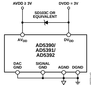
Figure 42. DV_{DD} first followed by AV_{DD}
