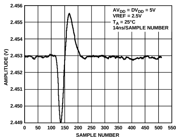
Figure 27. AD5390/AD5391/AD5392 Adjacent Channel Crosstalk
