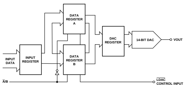
Figure 48. Toggle Mode Function
