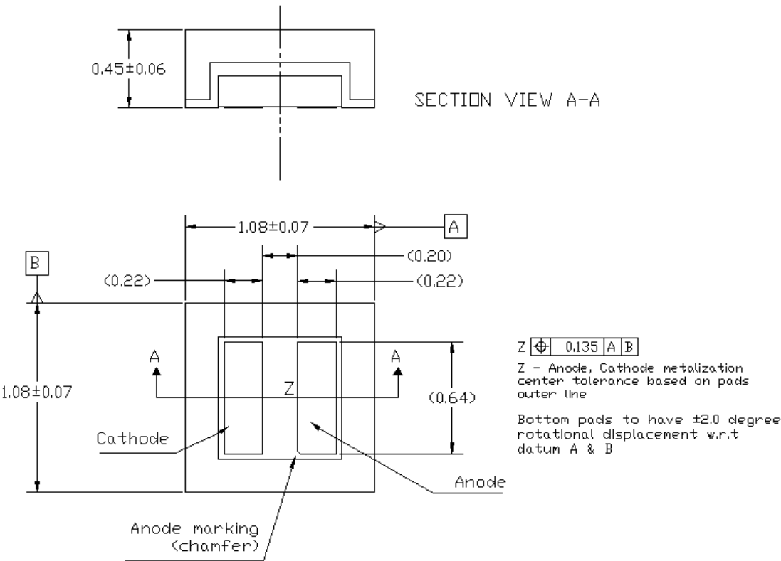
Figure 8: Mechanical dimensions for LUXEON FlipChip White 05.
