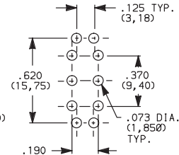
PC MOUNTING
