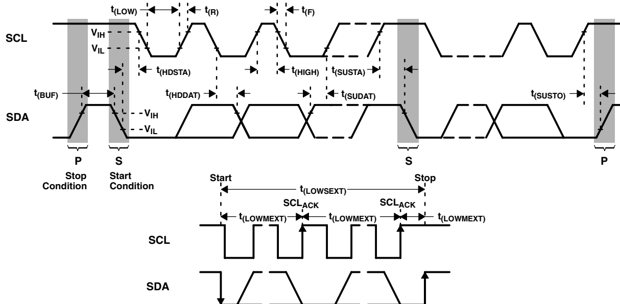
Figure 1. Timing Diagrams
